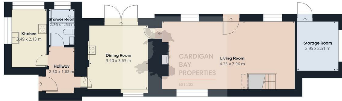
Floor 0
